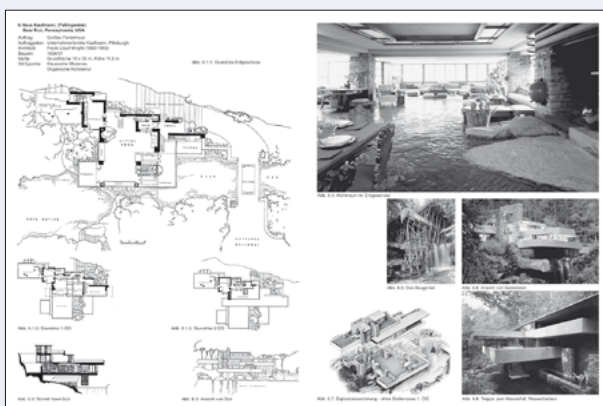
Haus Kaufmann (Fallingwater), Bear Run, Pennsylvania, USA (1936–37)
